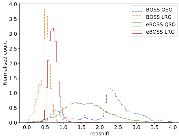
FIG. 1.— N(z) of eBOSS DR14 QSO and LRG compared to DR12 BOSS, demonstrating how eBOSS is filling in the redshift desert between z \sim 0.8 - 2.0 . Note that this shows only QSO and LRG targets because no significant number of ELGs have been released in DR14. To convert from Normalized Count to number as a function of redshift, multiply by the total numbers (given in Table 1 for the full survey) times the bin size of dz = 0.04 .
